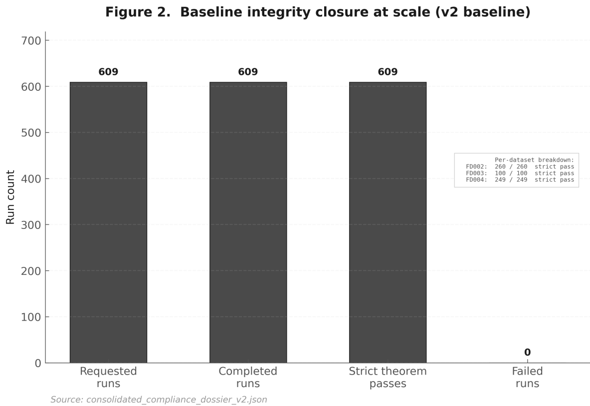
Figure 2. Baseline integrity closure at scale (v2 baseline). All 609 requested runs completed without failure, and all 609 passed strict theorem checks. The per-dataset breakdown (FD002: 260, FD003: 100, FD004: 249) confirms that integrity holds across diverse trajectory populations. Source artefact: consolidated_compliance_dossier_v2.json .
